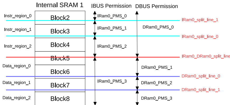
Figure 15.3-1. Split Lines for Internal SRAM1
