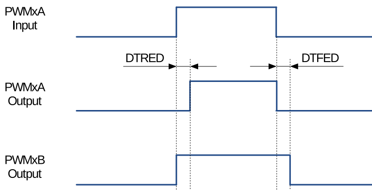
Figure 36.3-24. Active High (AH) Dead Time Waveforms
