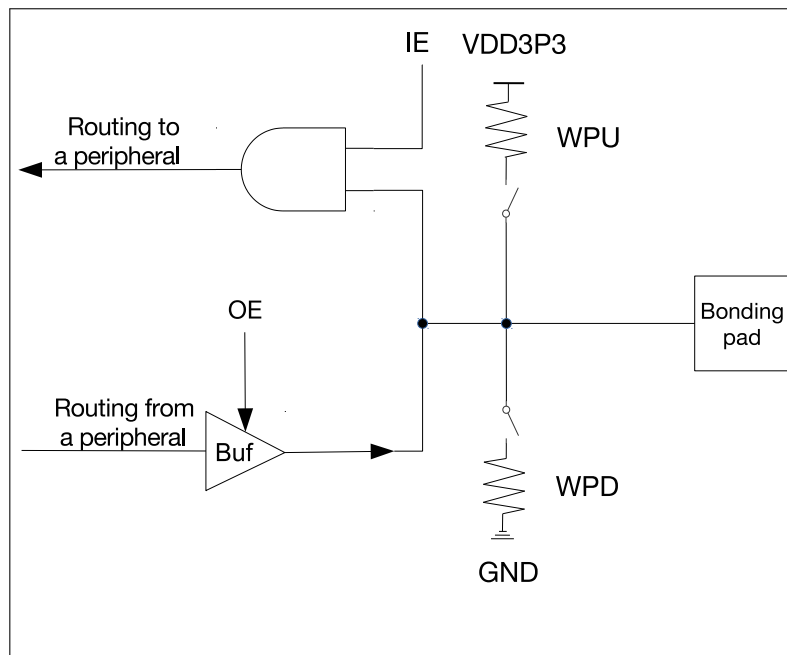
Figure 6.3-2. Internal Structure of a Pad
