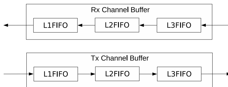
Figure 3.4-2. Channel Buffer
