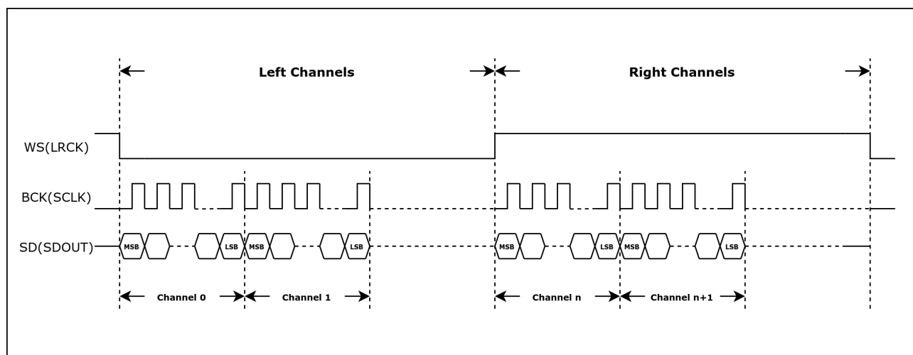
Figure 28.5-2. TDM MSB Alignment Standard Timing Diagram
