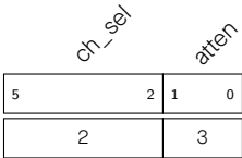
Figure 39.3-9. SAR ADC1 cmd0 Configuration
