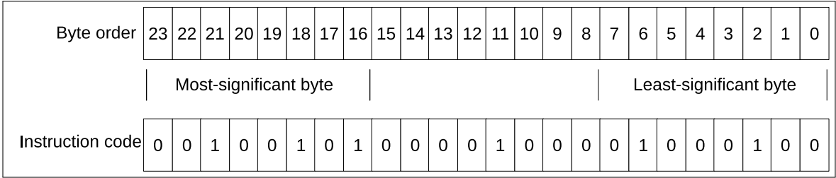
Figure 1.4-3. EE.ZERO.QACC in Little-Endian Byte Order
