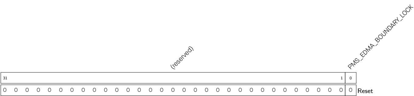
Register 15.68. PMS_EDMA_BOUNDARY_LOCK_REG (0x02A8)
