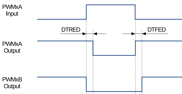
Figure 36.3-25. Active Low (AL) Dead Time Waveforms
