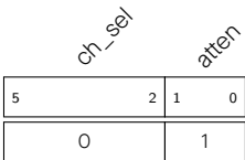
Figure 39.3-10. SAR ADC1 cmd1 Configuration
