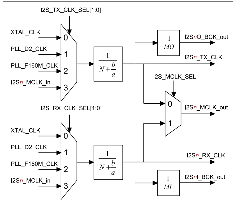
Figure 28.6-1. I2S n Clock
