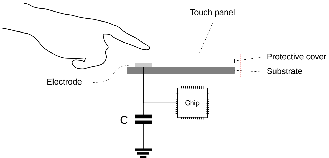
Figure 39.2-1. Touch Sensor
