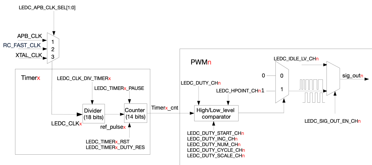
Figure 35.3-1. LED PWM Generator Diagram
