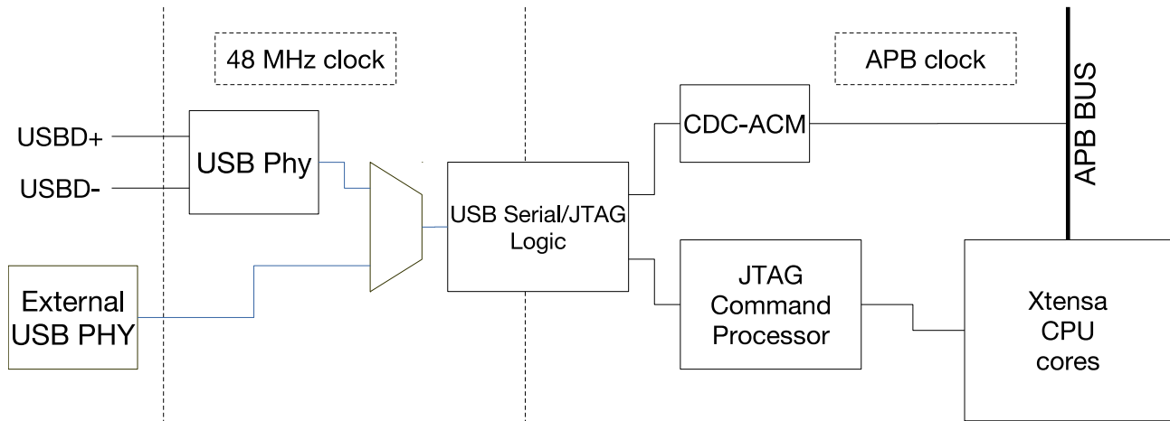
Figure 33.2-1. USB Serial/JTAG High Level Diagram
