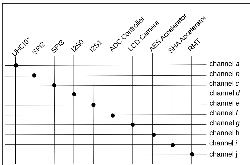
Figure 4.3-2. Peripherals/modules that can work with GDMA
