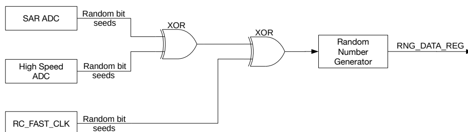
Figure 25.3-1. Noise Source
