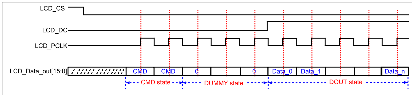
Figure 29.4-3. LCD Timing (I8080 Format)
