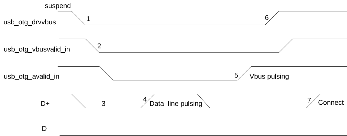
Figure 32.4-1. A-Device SRP
