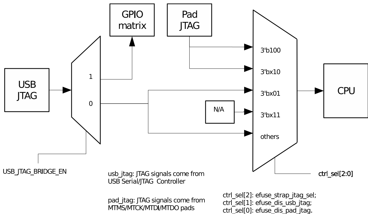
Figure 33.3-2. JTAG Routing Diagram
