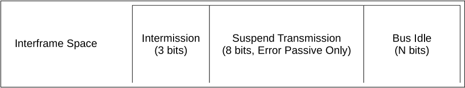
Figure 31.3-4. The Fields within an Interframe Space
