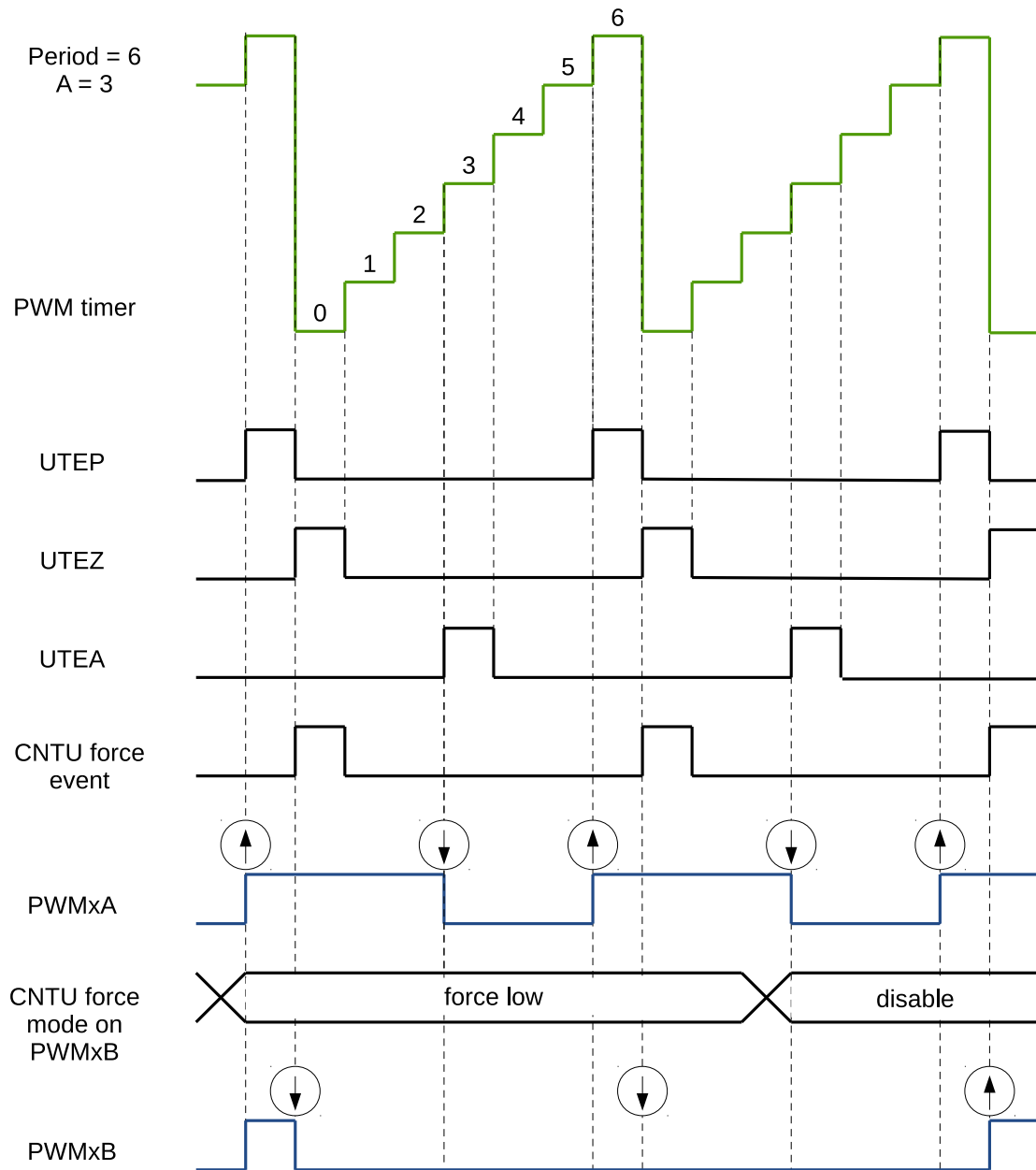
Figure 36.3-20. Example of a CNTU Software-Force Event on PWMxB
