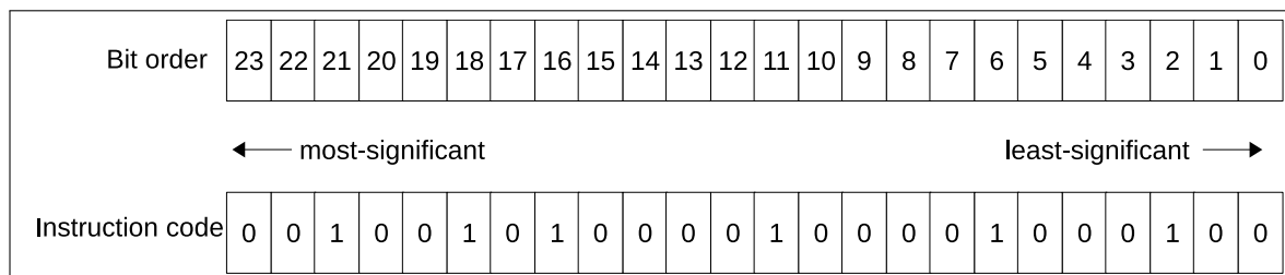
Figure 1.4-1. EE.ZERO.QACC in Little-Endian Bit Order
