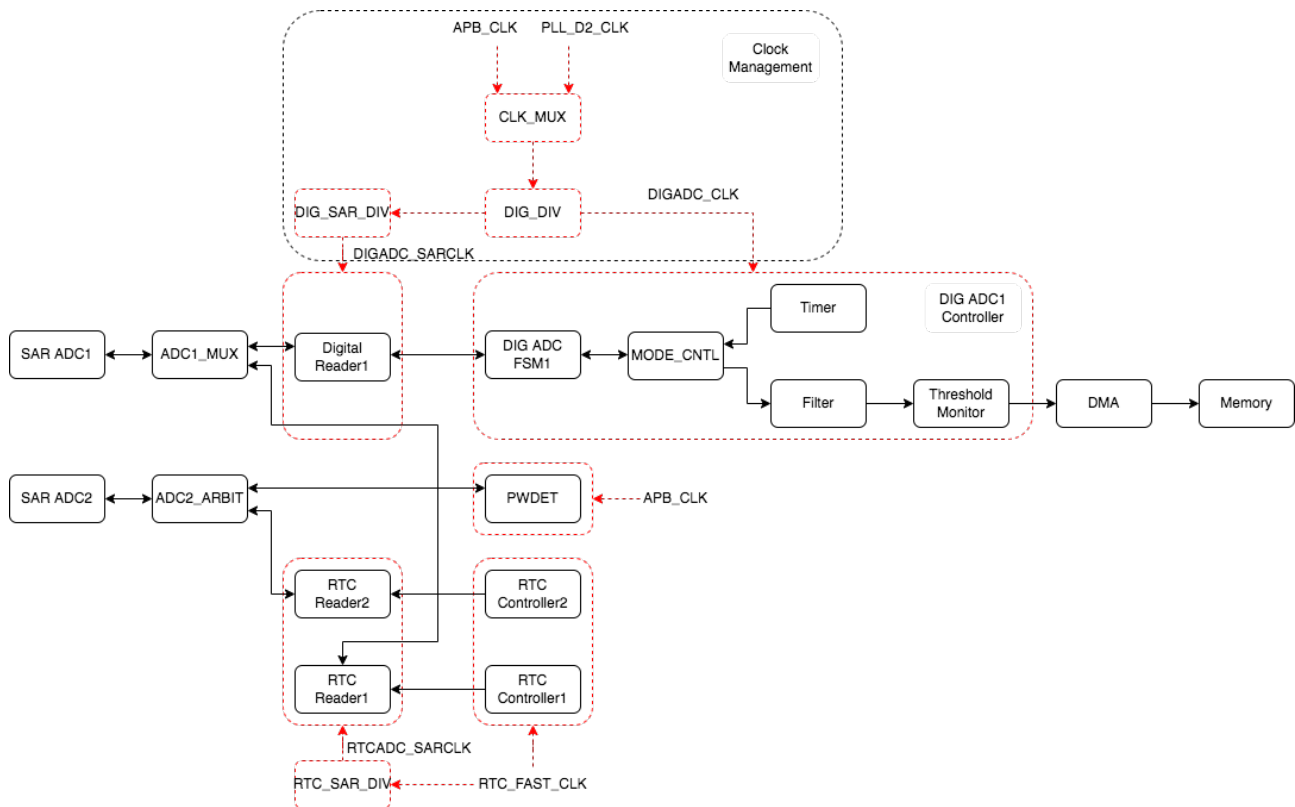
Figure 39.3-2. SAR ADC Architecture
