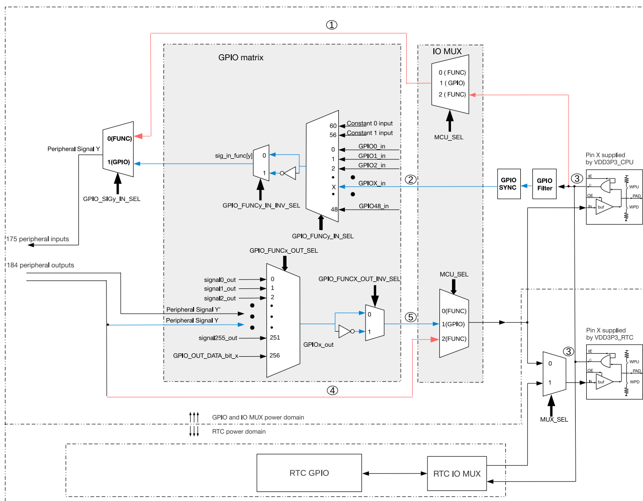
Figure 6.3-1. Architecture of IO MUX, RTC IO MUX, and GPIO Matrix
