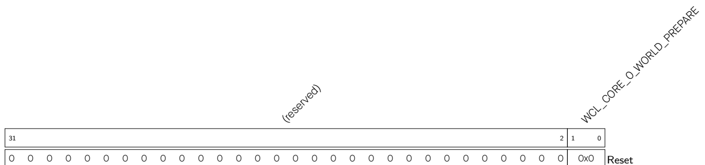
Register 16.9. WCL_CORE_O_World_PREPARE_REG (0x0144)
