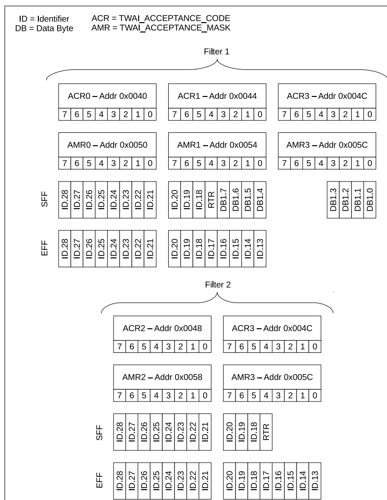
Figure 31.5-3. Dual Filter Mode
