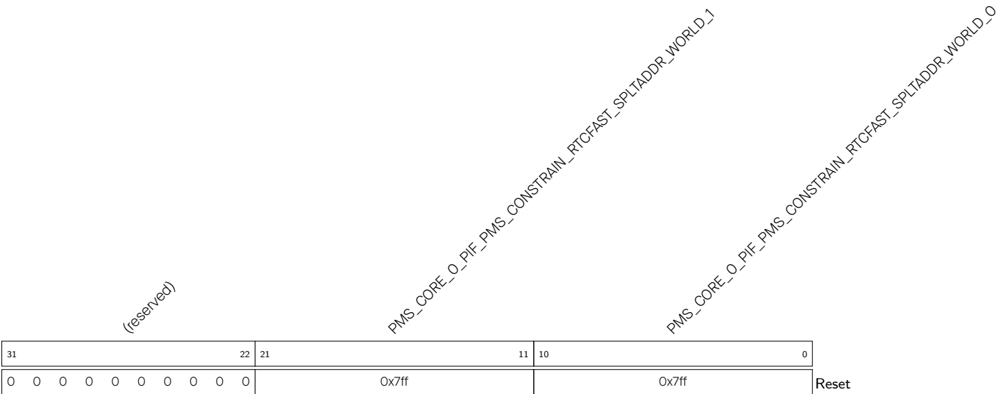
Register 15.51. PMS_CORE_O_PIF_PMS_CONSTRRAIN_9_REG (0x0148)
