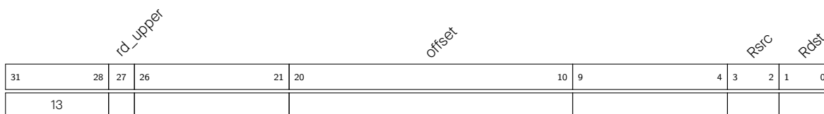
Figure 2.5-10. Instruction Type - LD
