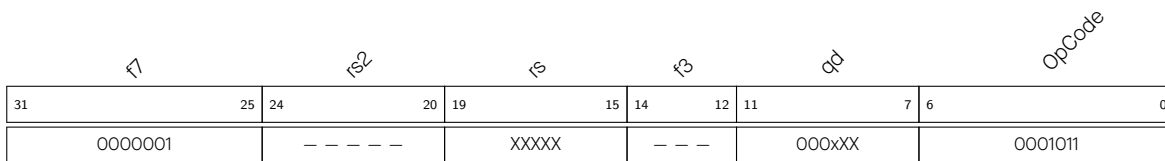
Figure 2.6-3. Interrupt Instruction - setq qd,rs
