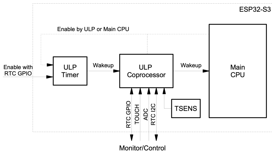
Figure 2.1-1. ULP Coprocessor Overview
