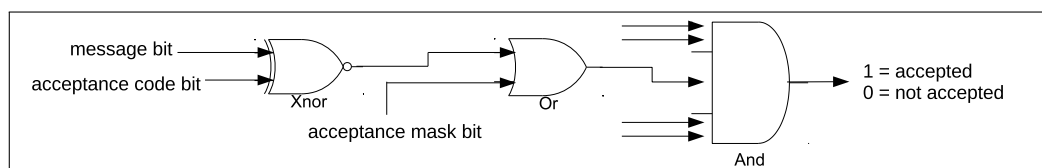
Figure 31.5-1. Acceptance Filter
