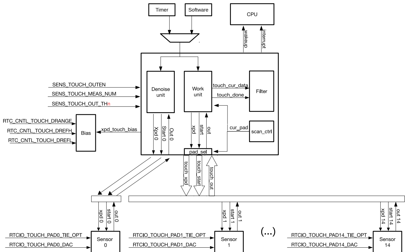
Figure 39.2-4. Touch FSM Structure
