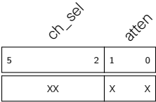
Figure 39.3-8. Pattern Table Entry
