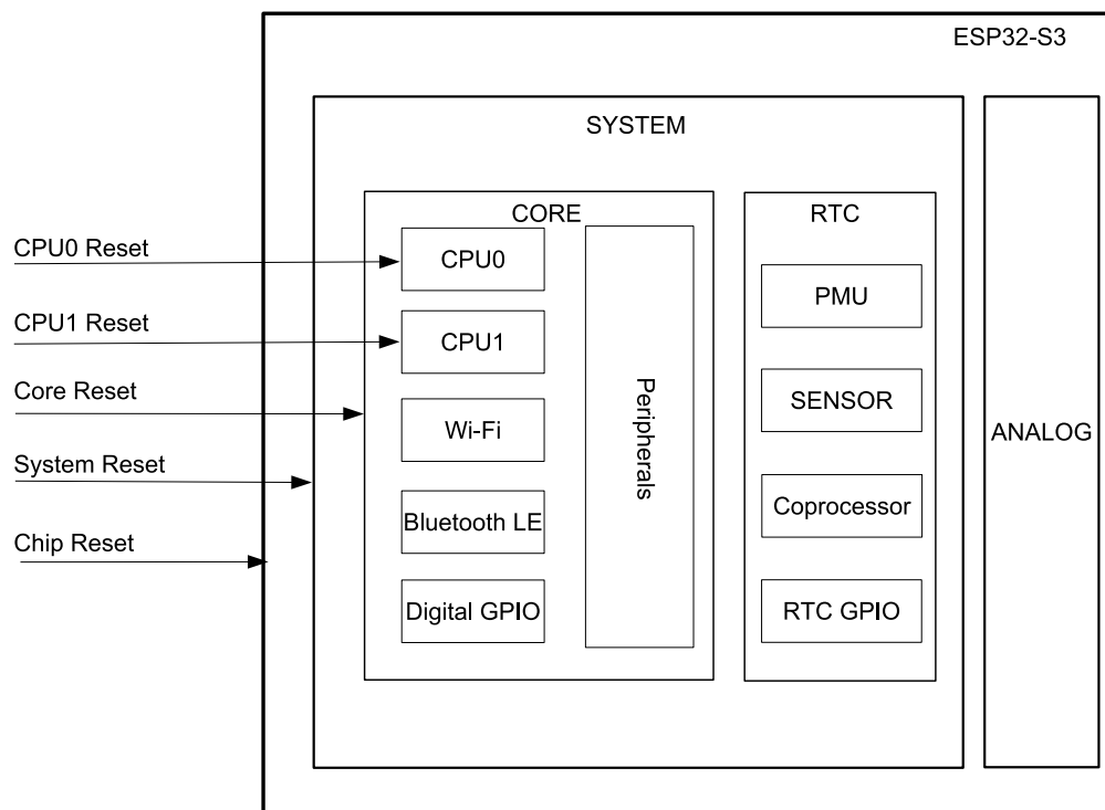
Figure 7.1-1. Reset Levels
