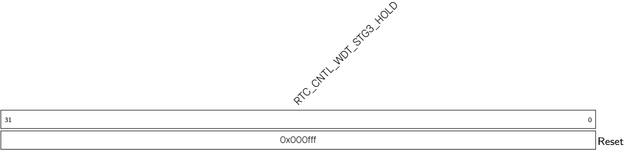
Register 10.36. RTC_CNTL_RTC_WDTCONFIG4_REG (0x00A8)
