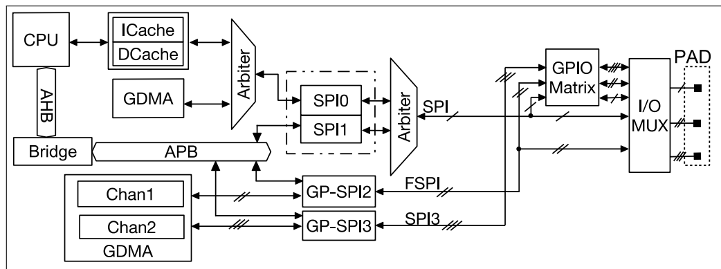
Figure 30.4-1. SPI Module Overview
