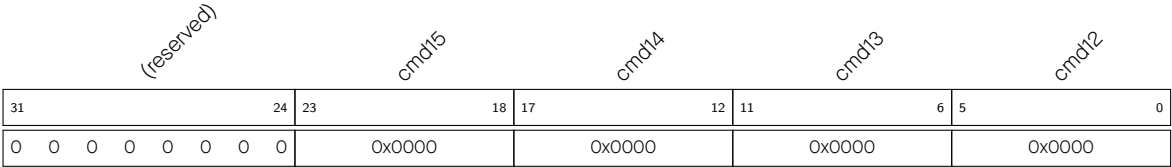
Figure 39.3-7. APB_SARADC_SAR1_PATT_TAB4_REG and Pattern Table Entry 12 - Entry 15
