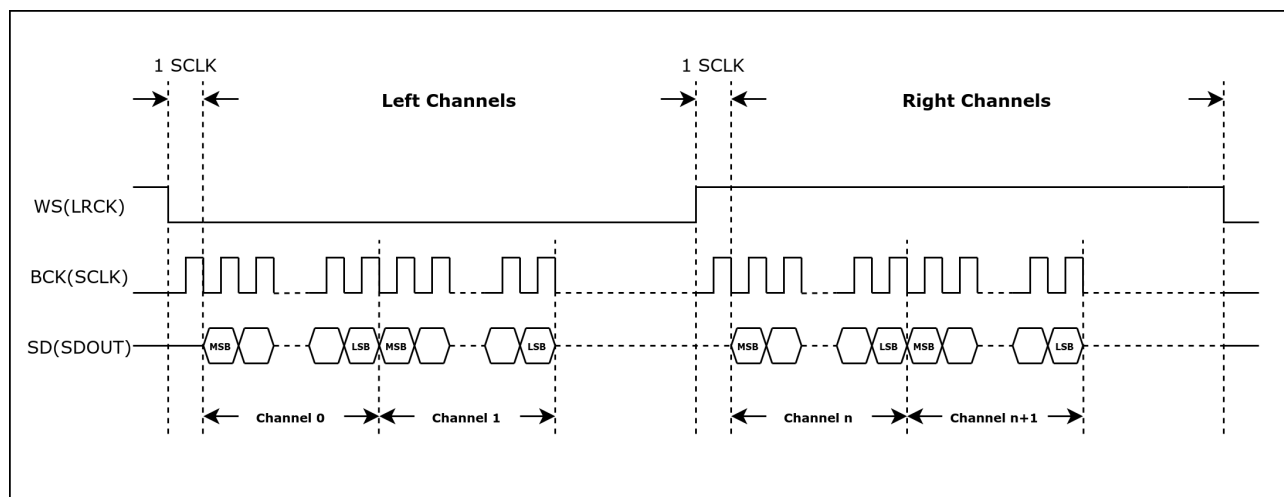
Figure 28.5-1. TDM Philips Standard Timing Diagram
