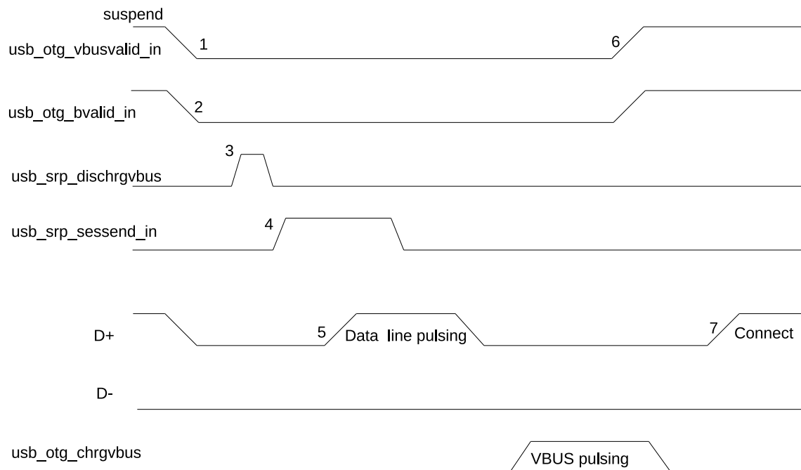
Figure 32.4-2. B-Device SRP
