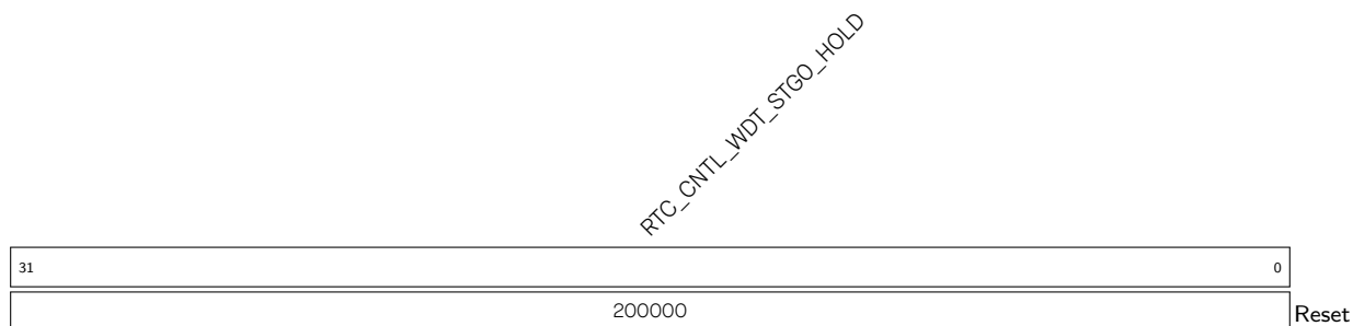
Register 10.33. RTC_CNTL_RTC_WDTCONFIG1_REG (0x009C)
