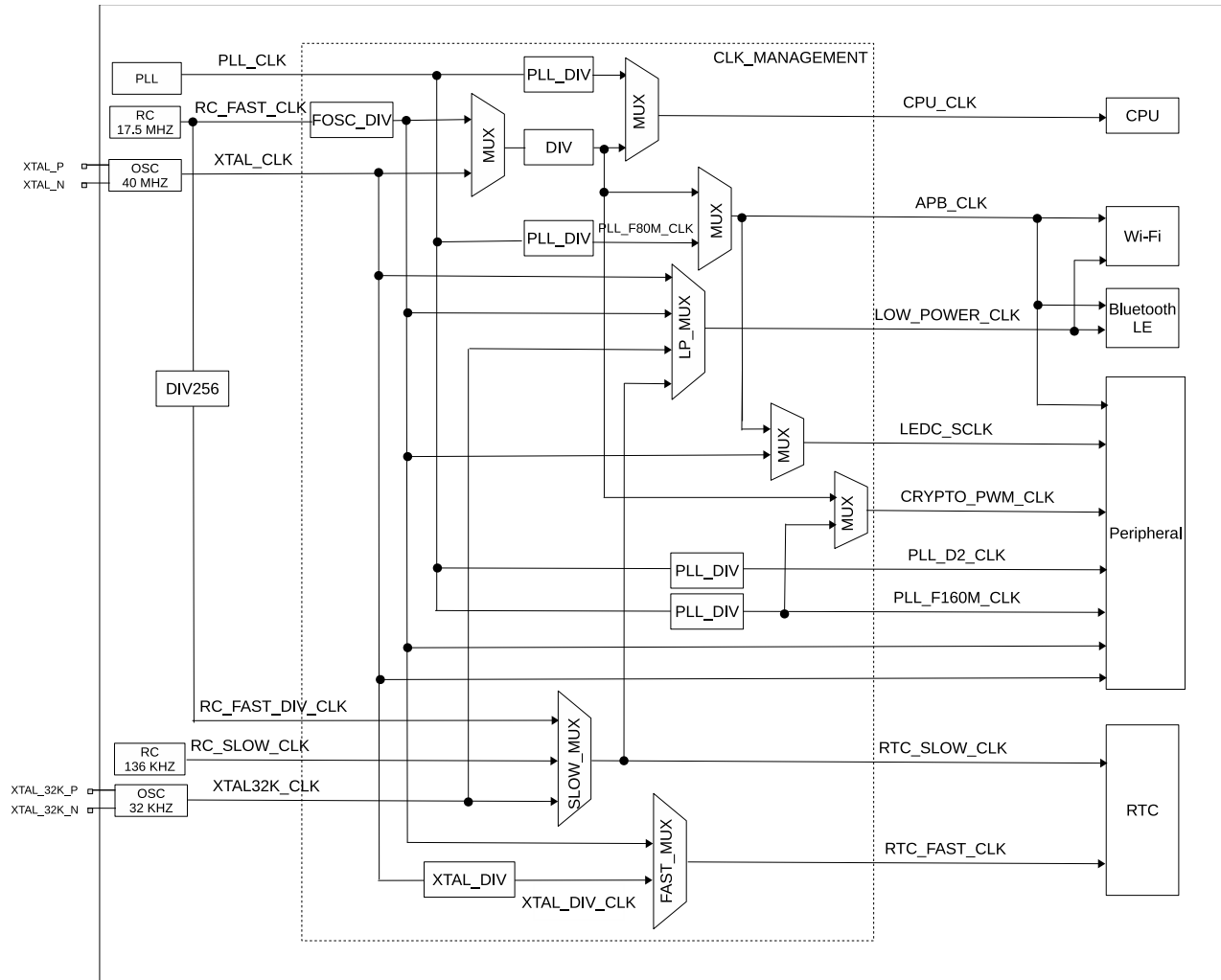
Figure 7.2-1. Clock Structure
