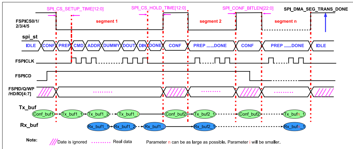
Figure 30.5-9. Configurable Segmented Transfer in DMA-Controlled Master Mode
