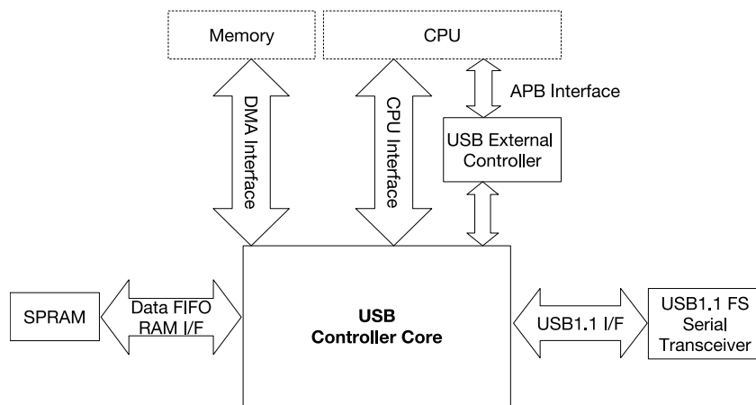
Figure 32.3-1. OTG_FS System Architecture
