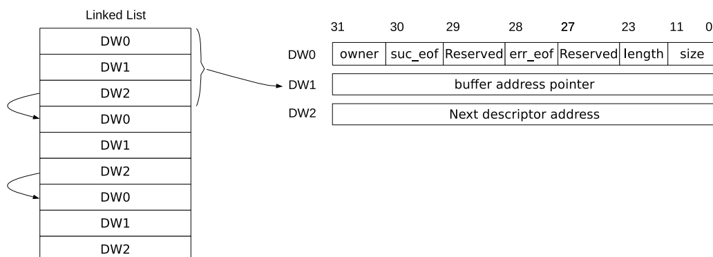
Figure 3.4-1. Structure of a Linked List
