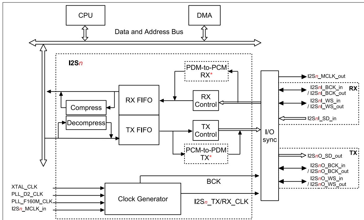
Figure 28.4-1. ESP32-S3 I2S System Diagram
