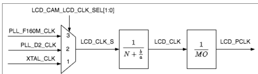
Figure 29.3-2. LCD Clock
