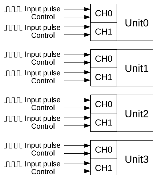
Figure 38.0-1. PCNT Block Diagram
