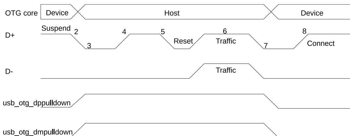
Figure 32.4-4. B-Device HNP
